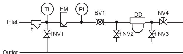
Sampling System Diagram
