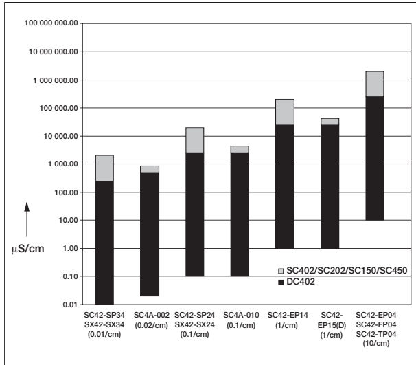
Measuring range as function of the cell constant
