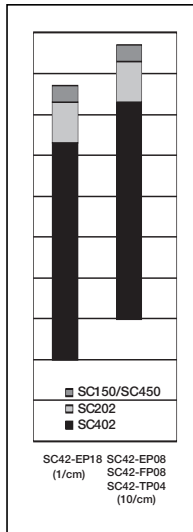
Measuring range as function of the cell constant
